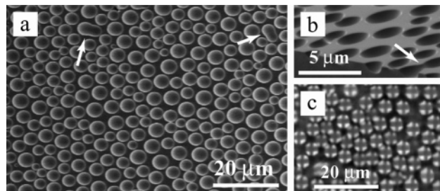
Figure 2. Concave patterns. (a) SEM image of a nontilted monolith. (b) SEM image of a tilted monolith. The arrows in (a) and (b) indicate elongated depressions templated by fused vesicles. (c) Virtual images obtained using a concave surface pattern as a microlens array from a single cross of 20 mm length and 2 mm line width (see Figure S1 in Supporting Information for the explanation of the simultaneous observation of concave depression bottoms and the images of the cross).
